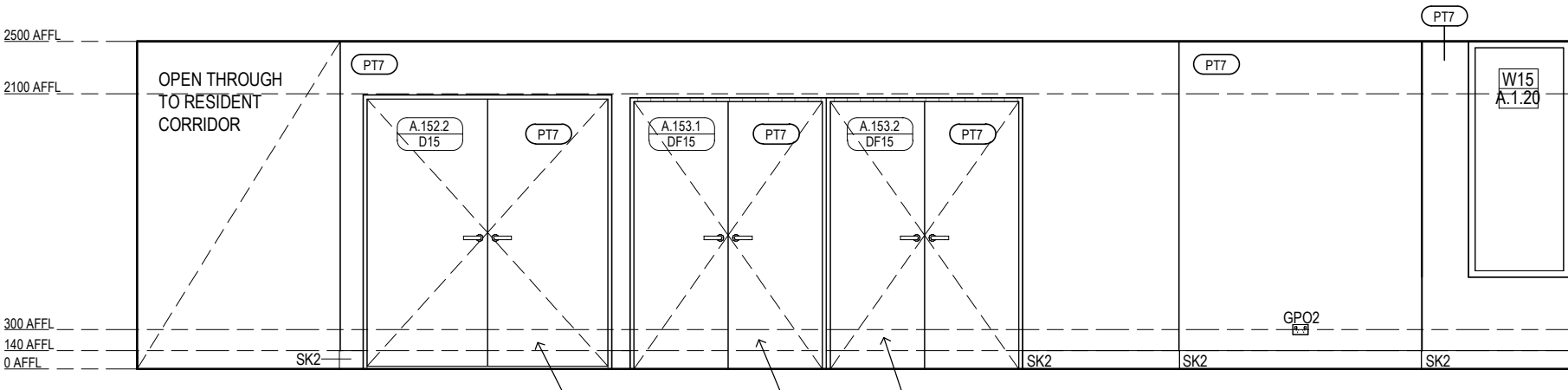
ILA L1 + L2 COMMUNAL SPACE ELEVATION 1 Scale 1 : 50
