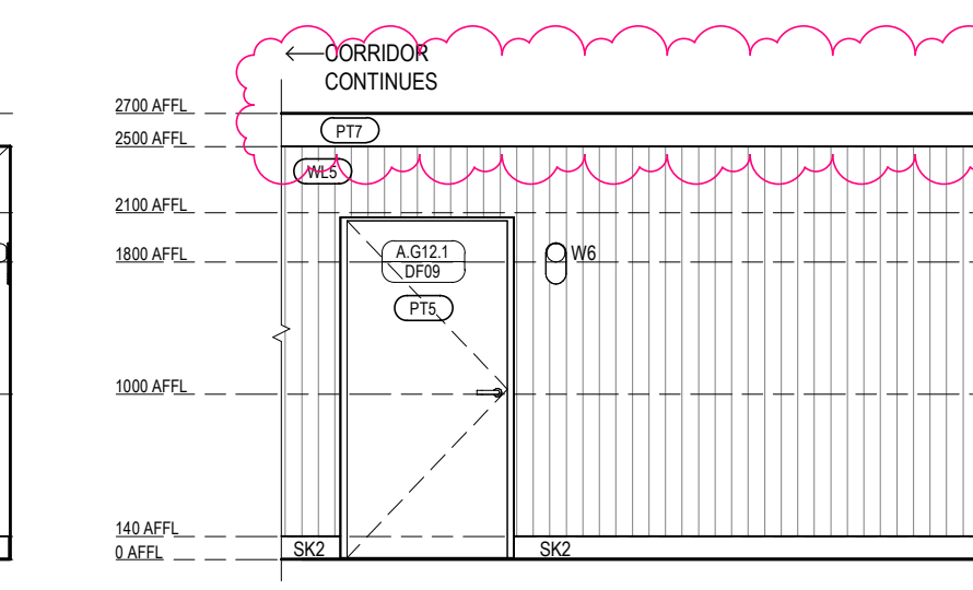
ILA Ground Floor Lift Lobby ELEVATION 3 Scale 1 : 50
