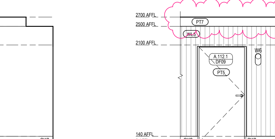
ILA L1 + L2 LIFT LOBBY ELEVATION 3 Scale 1 : 50
