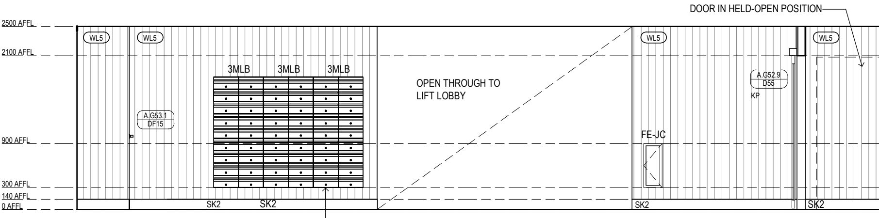
ILA GROUND FLOOR - FOYER ELEVATION 3 Scale 1 : 50
