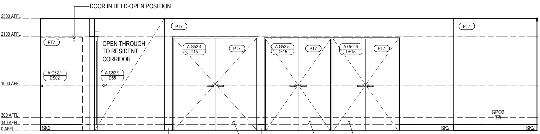
ILA GROUND FLOOR - FOYER ELEVATION 1 Scale 1 : 50
