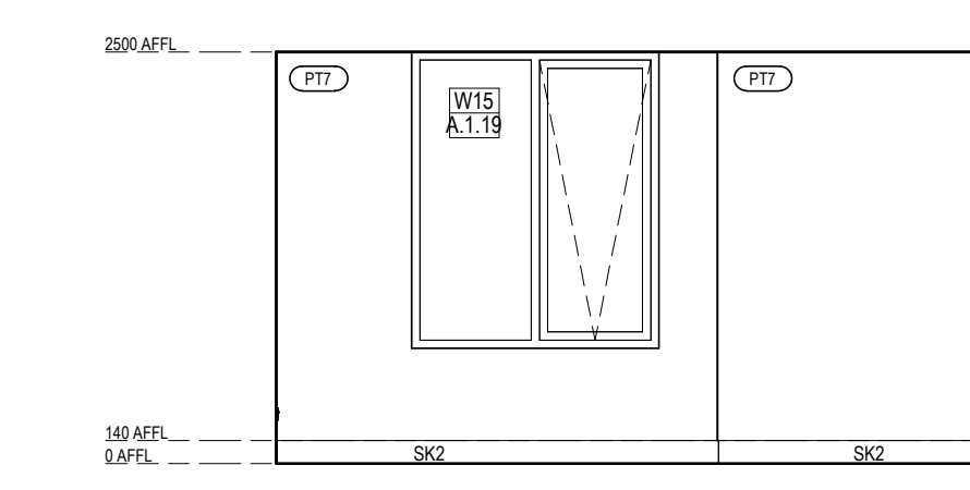
ILA L1 + L2 COMMUNAL SPACE ELEVATION 2 Scale 1 : 50
