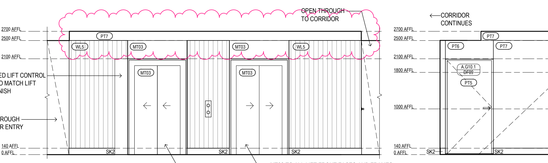
ILA GROUND FLOOR - LIFT LOBBY ELEVATION 1 Scale 1 : 50
