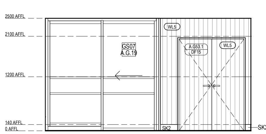
ILA GROUND FLOOR - FOYER ELEVATION 2 Scale 1 : 50
