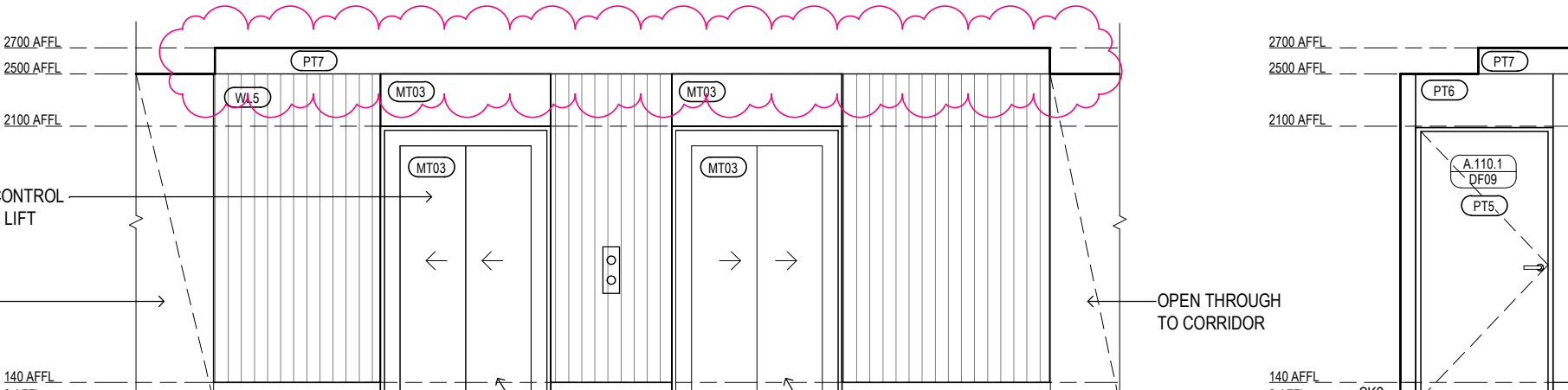
ILA L1 + L2 LIFT LOBBY ELEVATION 1 Scale 1 : 50
