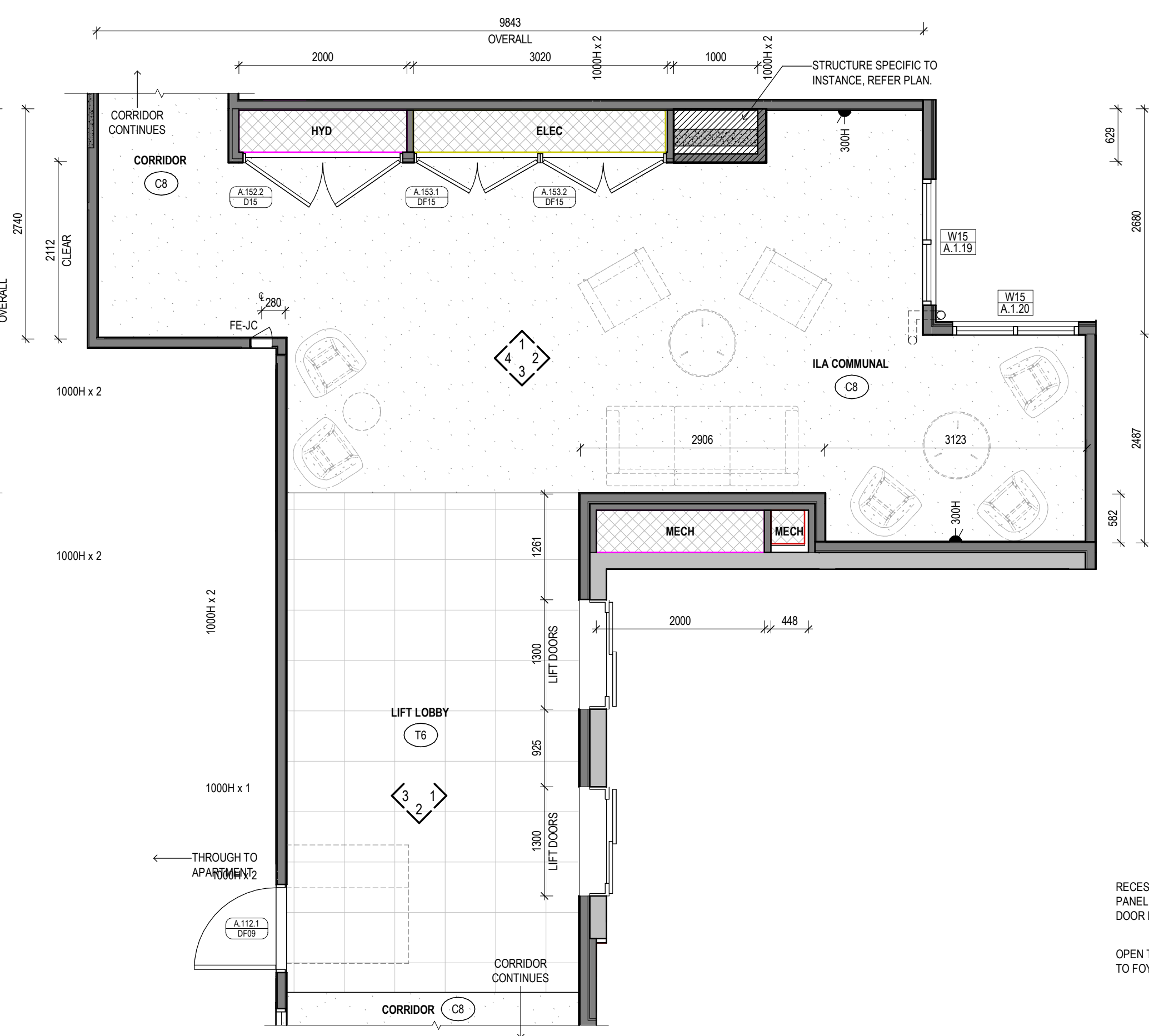
2 ILA L1+2 Lobby and Communal Space Scale 1 : 50
