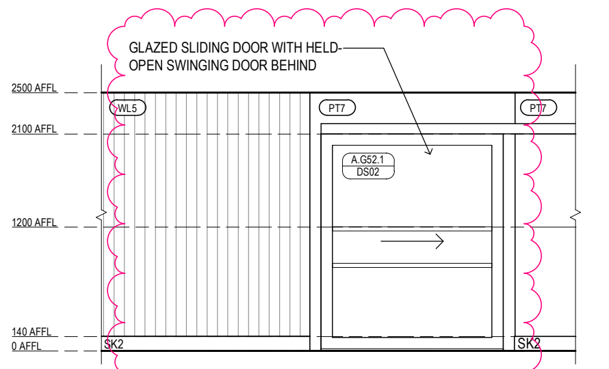
ILA GROUND FLOOR - FOYER ELEVATION 4 Scale 1 : 50
